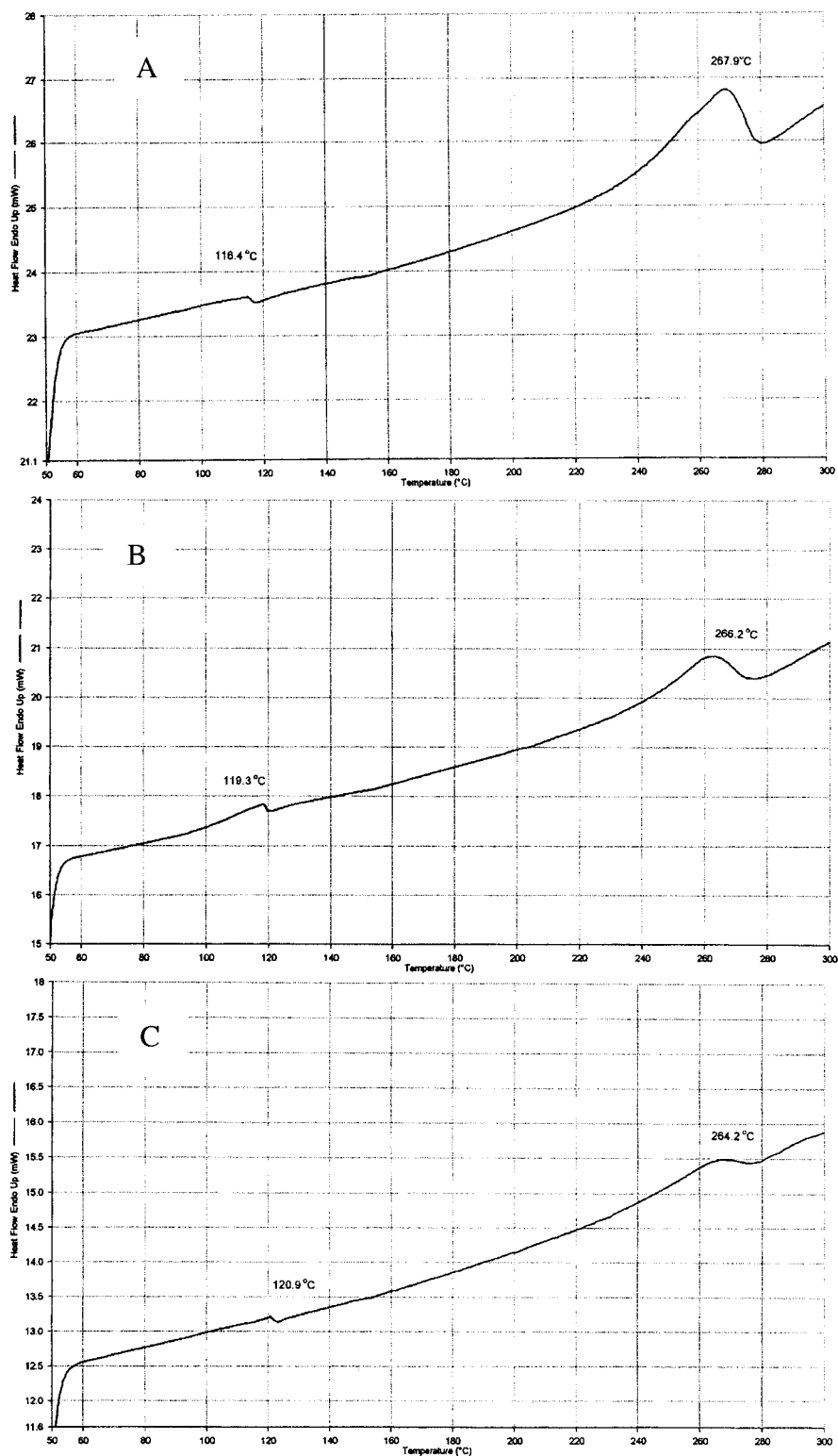
Figure 8 DSC thermograms of (A) the original FEP film, (B) the FEP-g-polystyrene film having a 40% degree of grafting, and (C) the FEP-g-polystyrene sulfonic acid membrane having a 40% degree of grafting.
